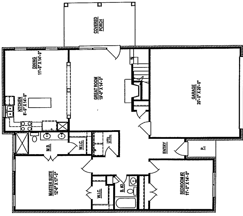
FIRST FLOOR
